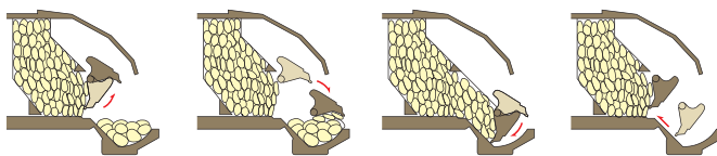
Loading System
