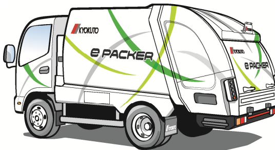
Press type electric refuse truck (Power feed system mounted)
