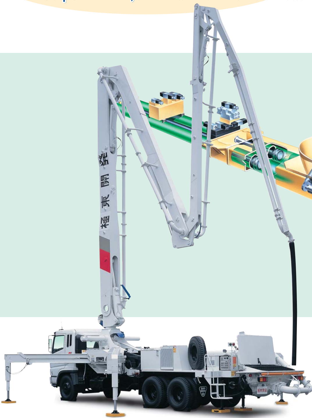
布料弯管有可预知磨损状况的观测凹槽设计 Piping elbow with wear-detect slit
